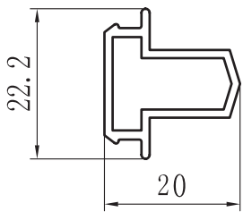
UNION 3/4 HOJAS ZX-6004
