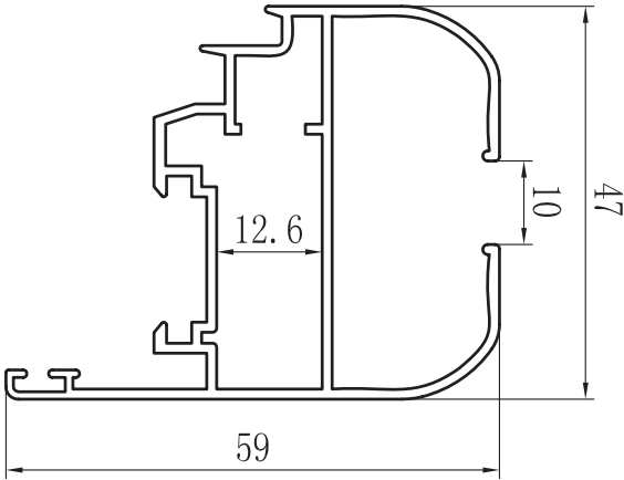
HOJA PRACTICABLE (VIDRIO 10) ZX-4003
