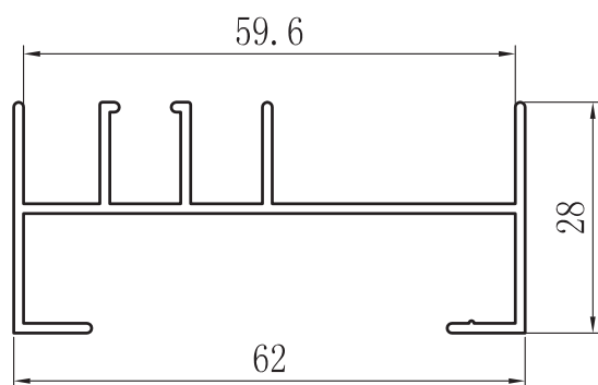
MARCO LATERAL ZX-6203
