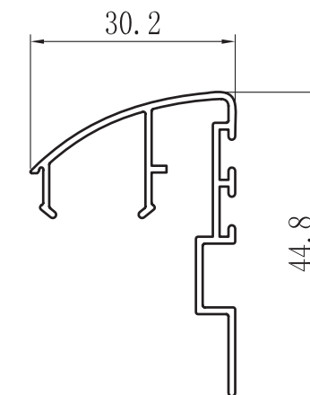
CLIP CRUCE EVO GRANDE ZX-6303
