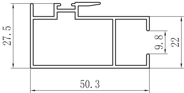
HOJA CENTRAL (VIDRIO 10) ZX-6207D
