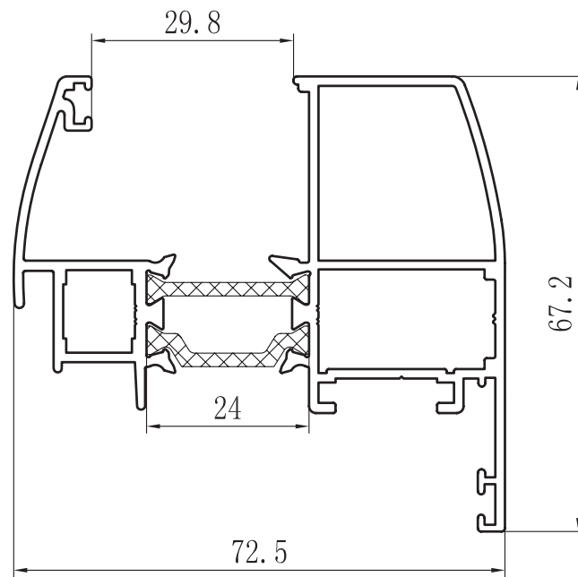
HOJA PRACTICABLE RPT ZX-6503BE
