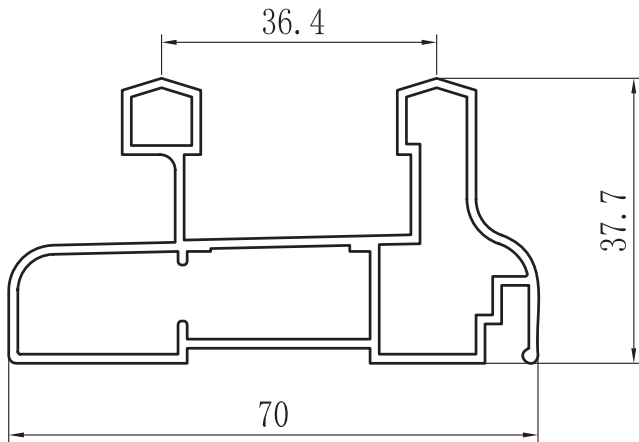
MARCO PERIMETRAL 70 (AUTOLIMPIABLE) ZX-6011
