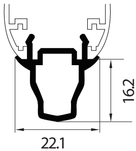
UNION 3/4 HOJAS GM-EVO ZX-08
