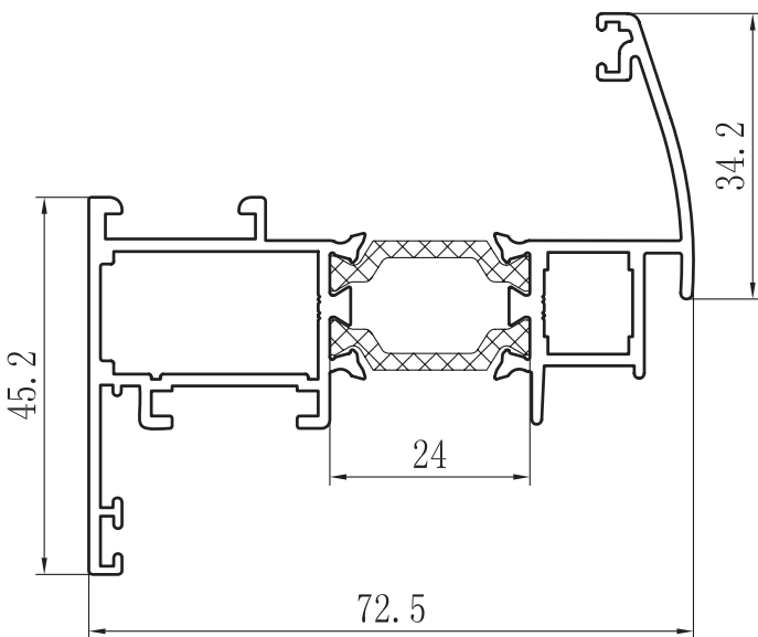
HOJA PRACTICABLE S/JUNQUILLO R.P.T. ZX-6503
