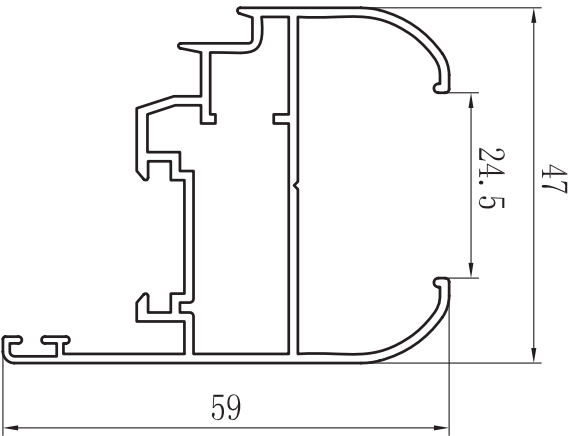
HOJA PRACTICABLE (VIDRIO 24.5) ZX-4003A
