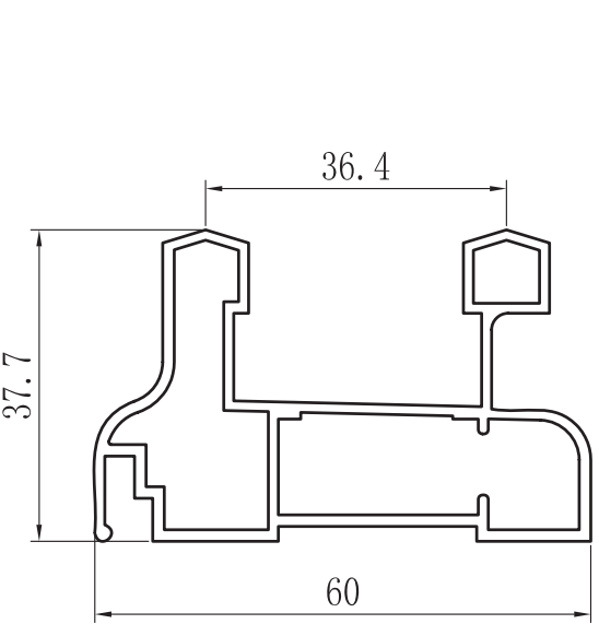
MARCO PERIMETRAL 60 (AUTOLIMPIABLE) ZX-6001
