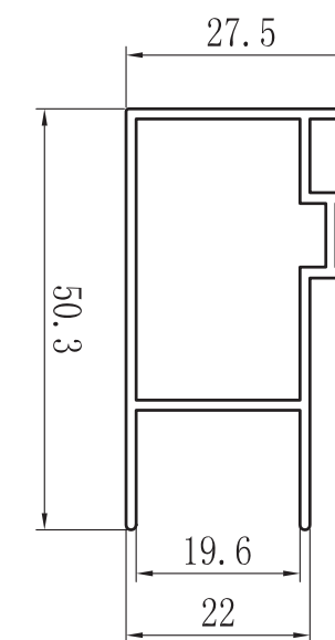
HOJA CENTRAL ZX-6207
