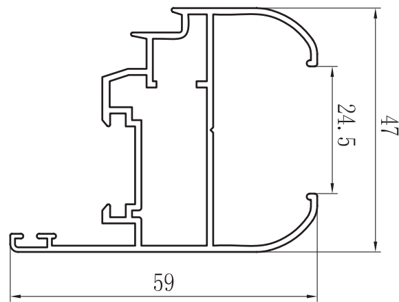
HOJA PRACTICABLE (VIDRIO 24.5) ZX-4003A
