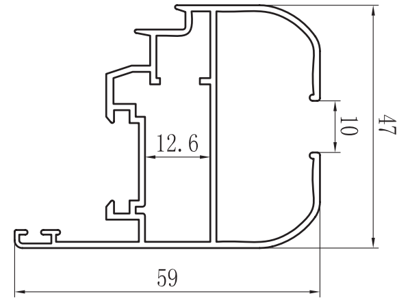
HOJA PRACTICABLE (VIDRIO 10) ZX-4003
