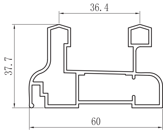
MARCO PERIMETRAL 60 (AUTOLIMPIABLE) ZX-6001
